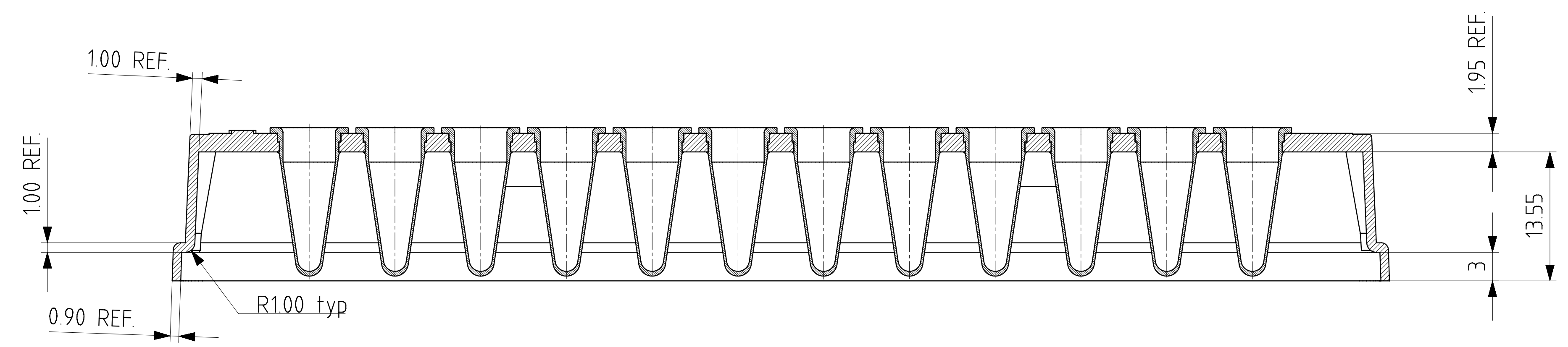
SECTION C-C
