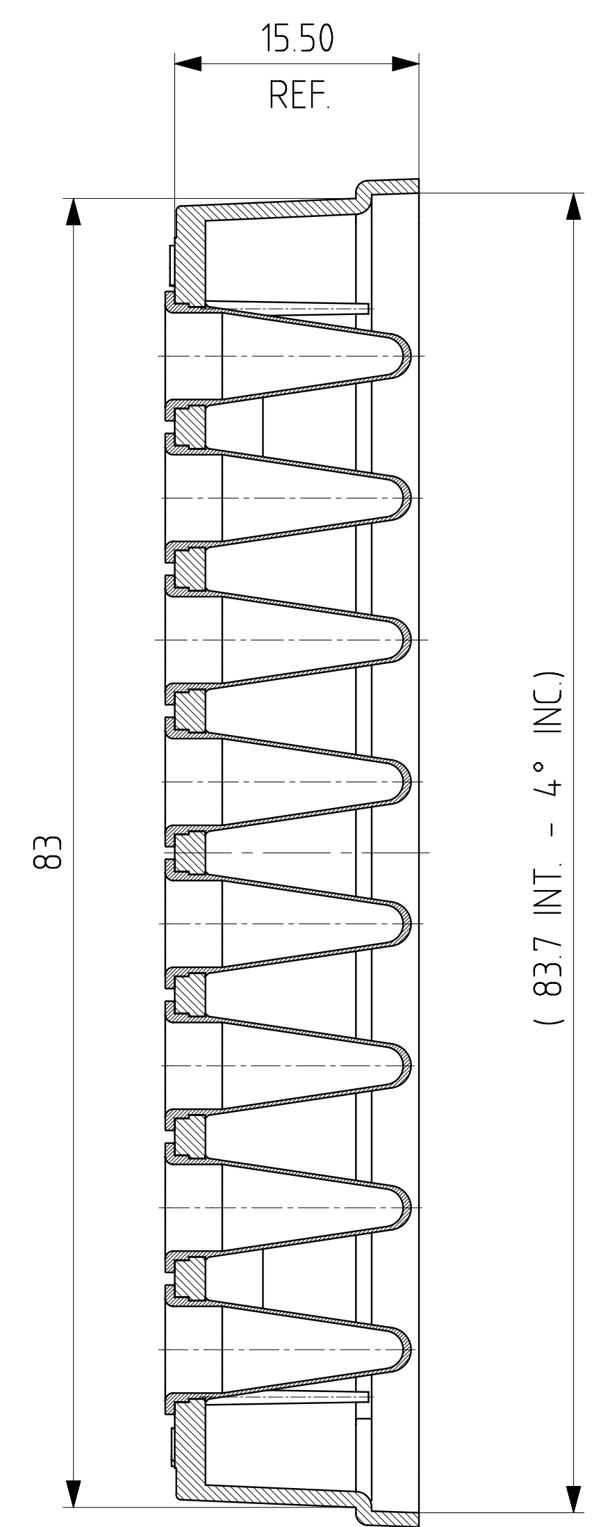
SECTION B-B
