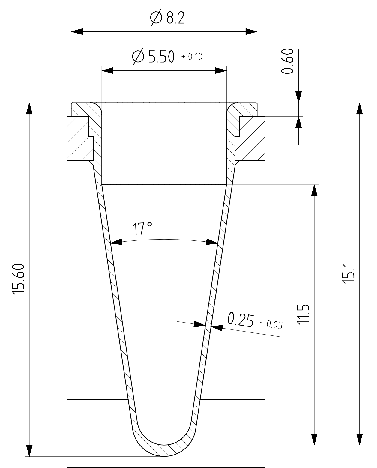
VIAL FORM 96pos. SCALE 10:1
