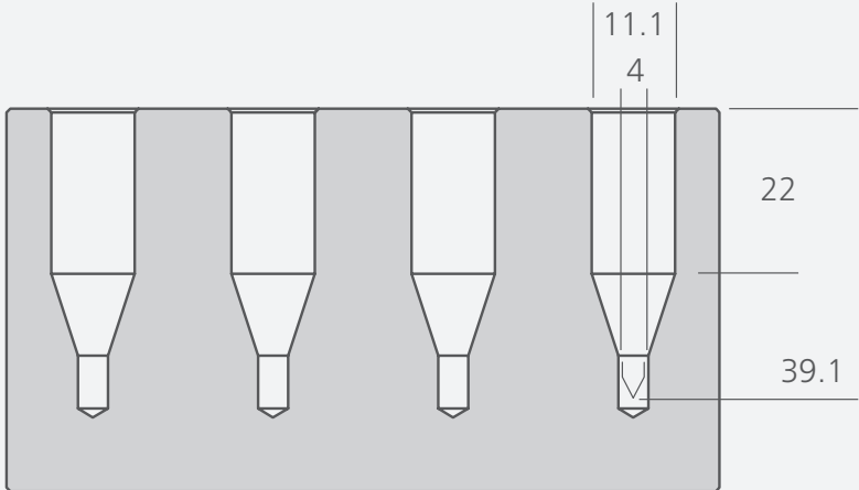
C-C (1:1)
